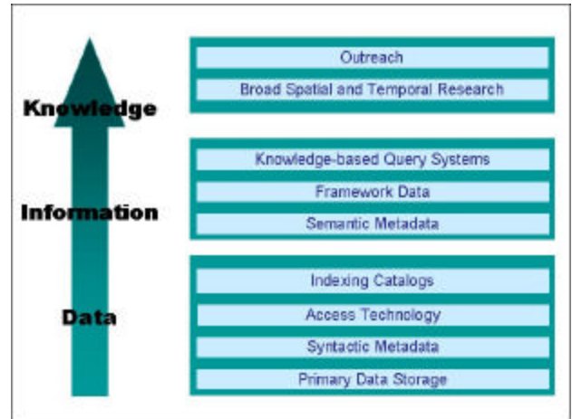
Figure 1. Component Model of Ecoinformatics Infrastructure
